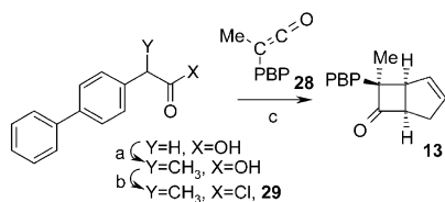
Scheme 6. Synthesis of alkene 13 . (a) n -BuLi (2 equiv), THF, −78 °C, then CH 3 I. (b) (COCl) 2 , CHCl 3 , 0–25 °C. (c) Et 3 N, 1,3-cyclopentadiene. (PBP = para -biphenyl).
