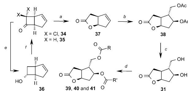
Scheme 8. Synthetic route to T-4 analogues. (a) MCPBA, NaHCO 3 , CH 2 Cl 2 , 25 °C; (b) (i). (CH 2 O) n , H 2 SO 4 , AcOH, 80 °C; (ii). Ac 2 O, DMAP, Pyr., CH 2 Cl 2 ; (c) NaOMe, MeOH; (d) RCOCl, Pyr., DMAP, CH 2 Cl 2 , 25 °C; (e) Bakers Yeast, Sucrose, water—3 days; (f) Jones reagent.
